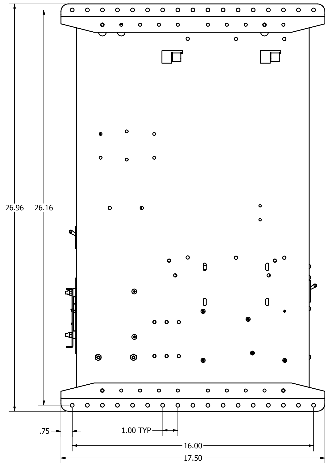
CLIPPER MOUNTING BRACKET DIMENSIONS
