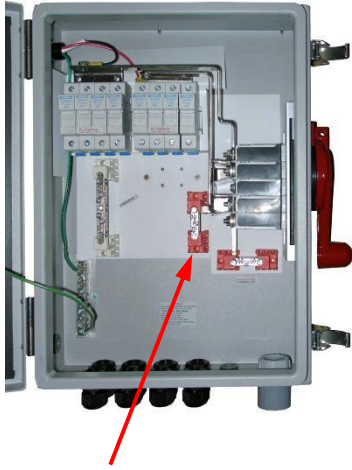
Step 4: Reinstall Positive block
