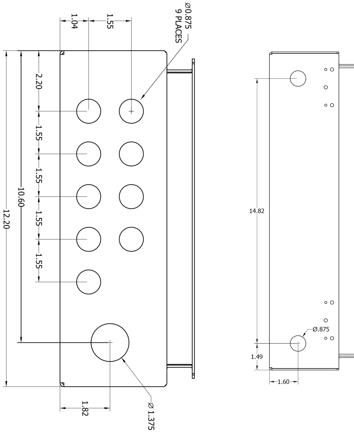
MNPV8HV Type 4X bottom and side knockout location and size
