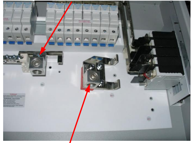
Remove PV positive Combined Out lug by removing nuts on breakers. It will be reinstalled in Step 4
