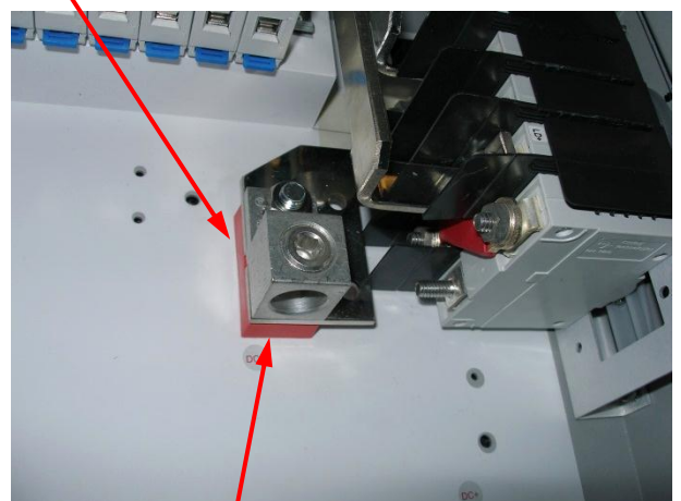
Reinstall PV positive output box lug in its original position using a 7/16” boxwrench. See torque chart on Page 5. Install sealed 10-32 X 3/8 screw through bottom into red insulator brass insert
