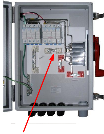
Step 5: Reinstall Negative block
