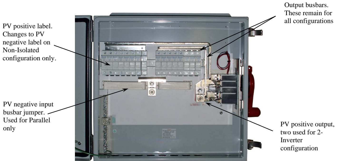
MNPV16HV Parallel configuration (default) 16-string Disconnecting Combiner
